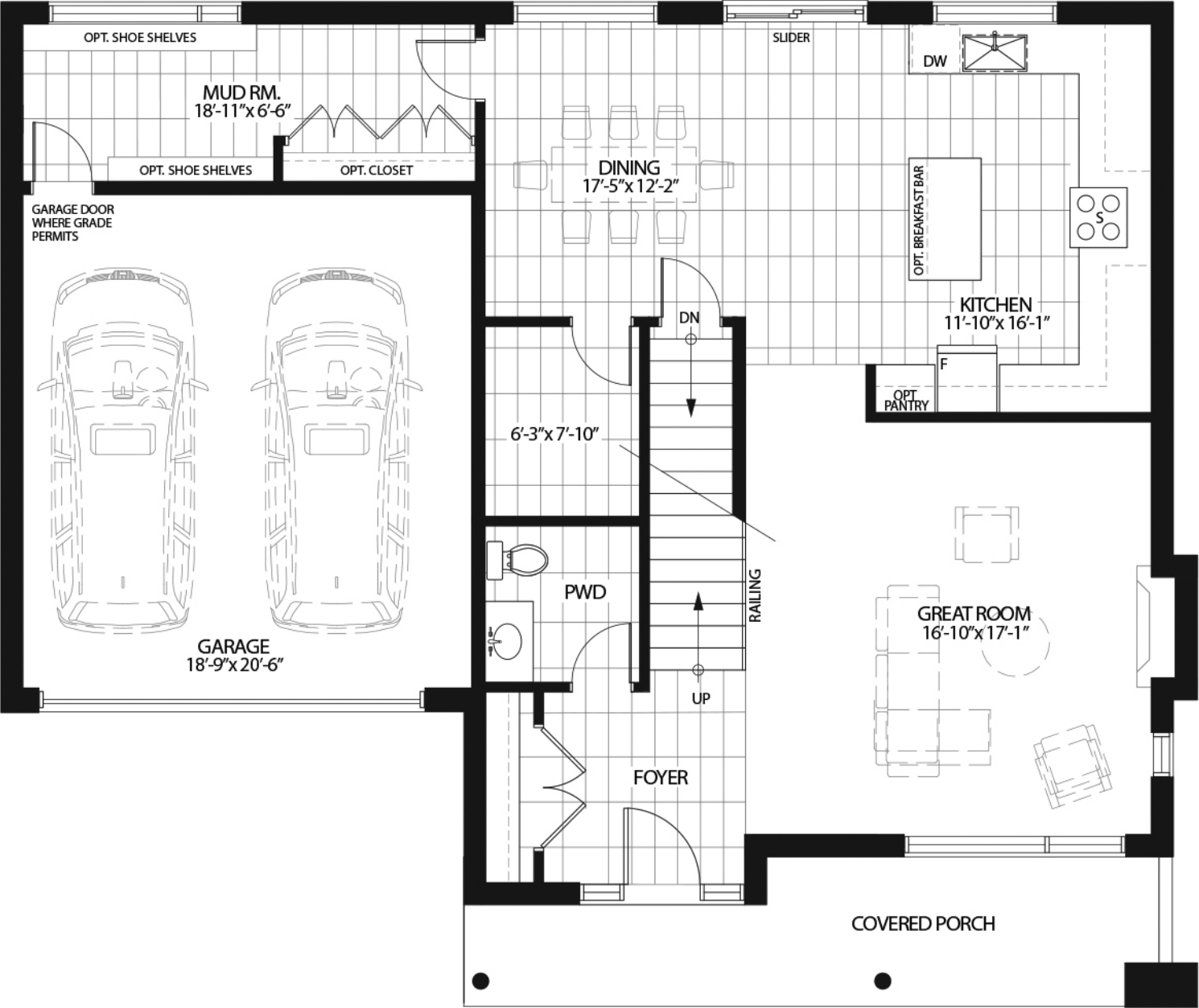
FIRST FLOOR
